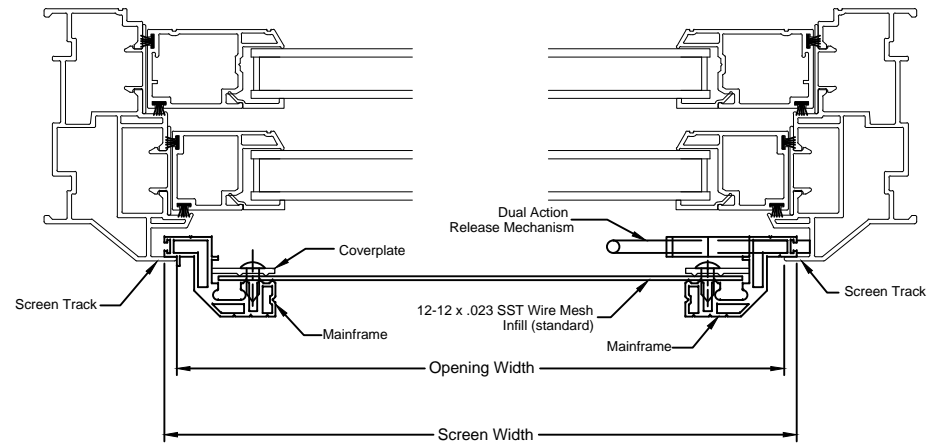
500-B Series Removable Mounted Into Screen Track
