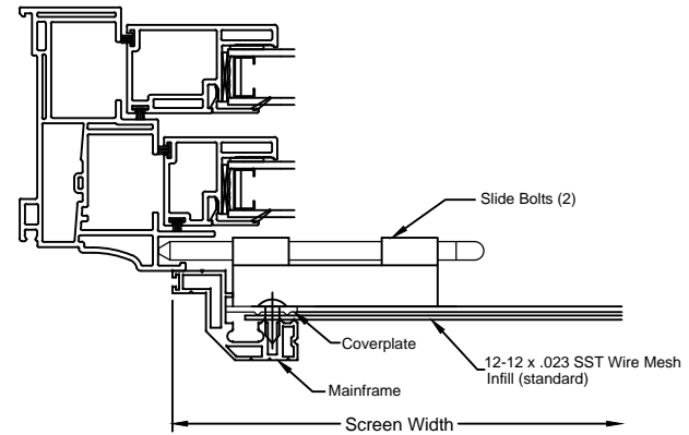
500-C Series Egressable Top Hinged Mounted to Window
