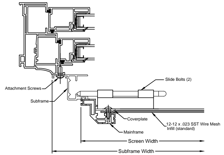
500-C Series Egressable Top Hinged w/ Subframe Mounted to Window
